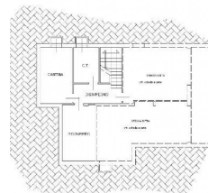
PIANO INTERRATO
